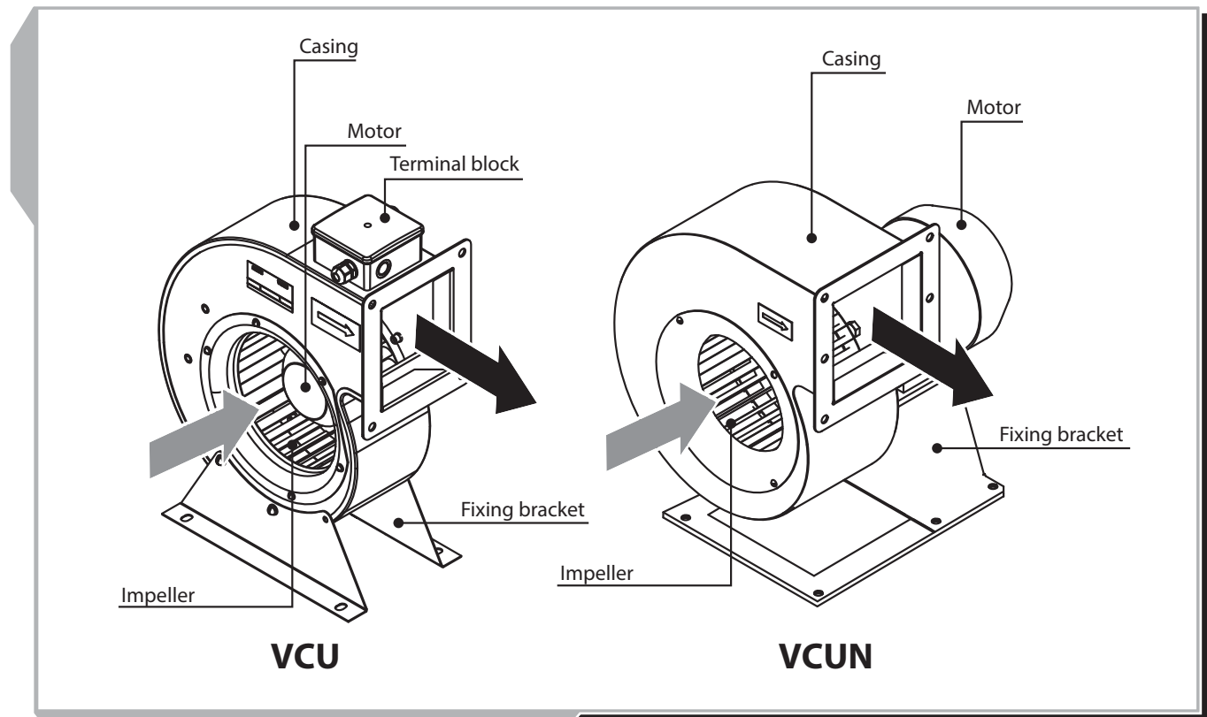
Fig. 4. Fan design and operating logic
