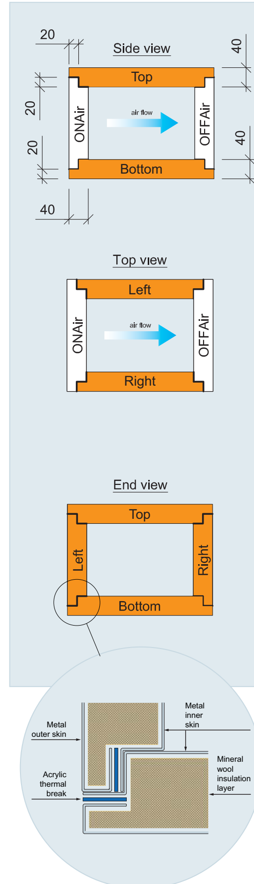
Frameless casing connection
