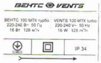
100 MTK turbo
