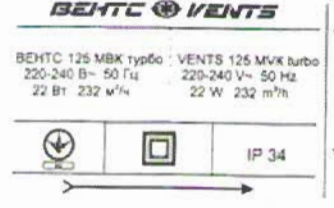
125 MBK turbo
