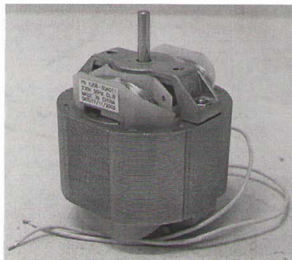
4. picture: Built in motor (Huanying YJ58-30A01)
