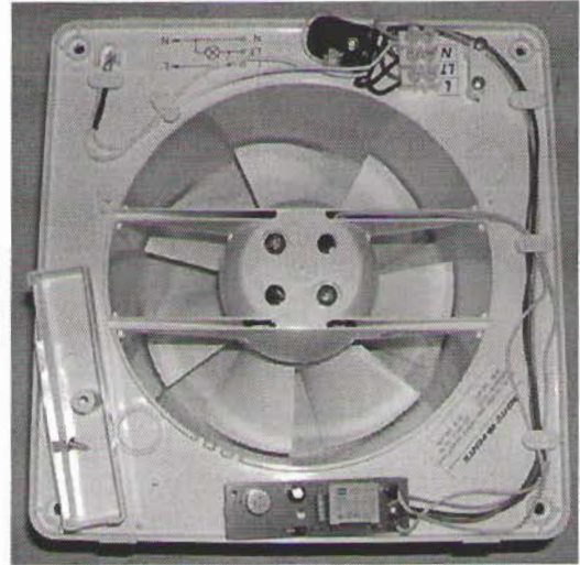
11. picture: Connection box with terminal, switch and timer of 'xxx' MVT turbo types
