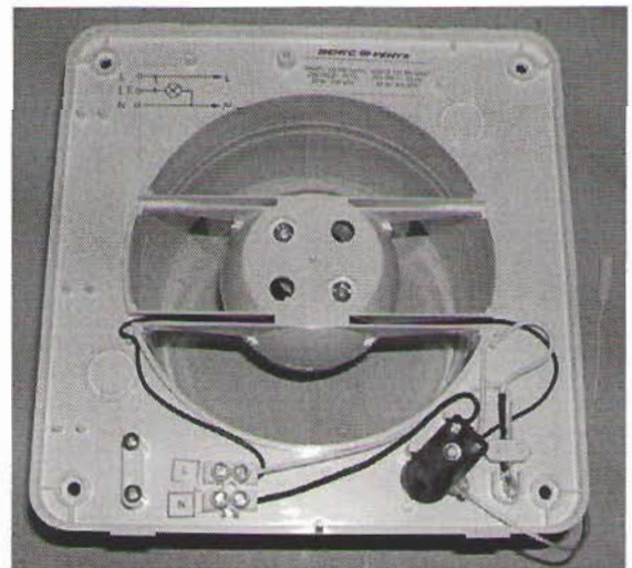
9. picture: Connection box with terminal and switch of 'xxx' MV turbo types
