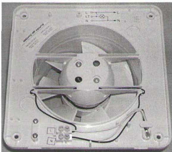
8. picture: Connection box with terminal of 'xxx' M turbo types
