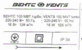
100 MVT turbo
