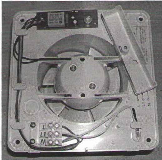
10. picture: Connection box with terminal and timer of 'xxx' MT turbo types
